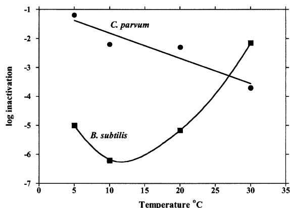
Fig. 1. Calculated temperature dependence of inactivation of B. subtilis spores and Cryptosporidium parvum oocysts in River Seine water after an ozone dosage of 2 mg l -1 at pH 8. Water quality: DOC 2.4 mg l -1 , alkalinity 3.8 mM, pH 8.
