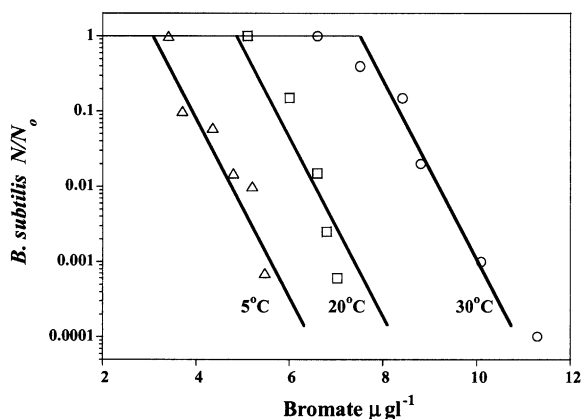
Fig. 3. Inactivation of B. subtilis spores and bromate formation during ozonation of Lake Zürich water at temperatures 5°C, 20°C and 30°C ( [\text{Br}^-]_0 = 30 \mu\text{g l}^{-1} , pH=7, DOC=1.4 mg l -1 , alkalinity 2.5 mM).
